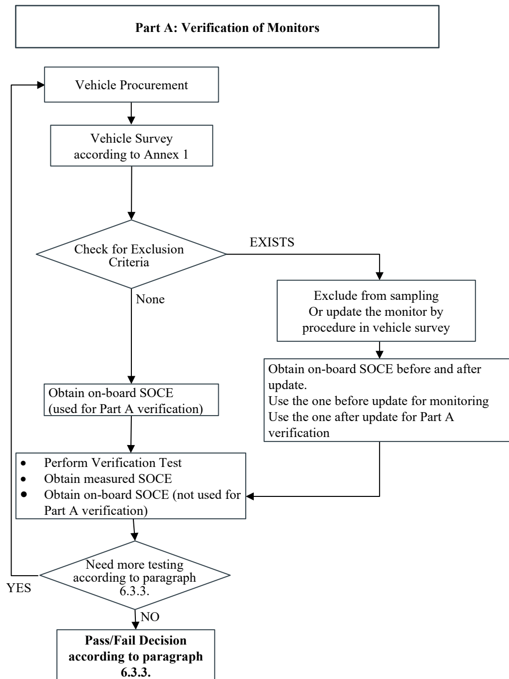
Flow chart for Part A: Verification of Monitors
