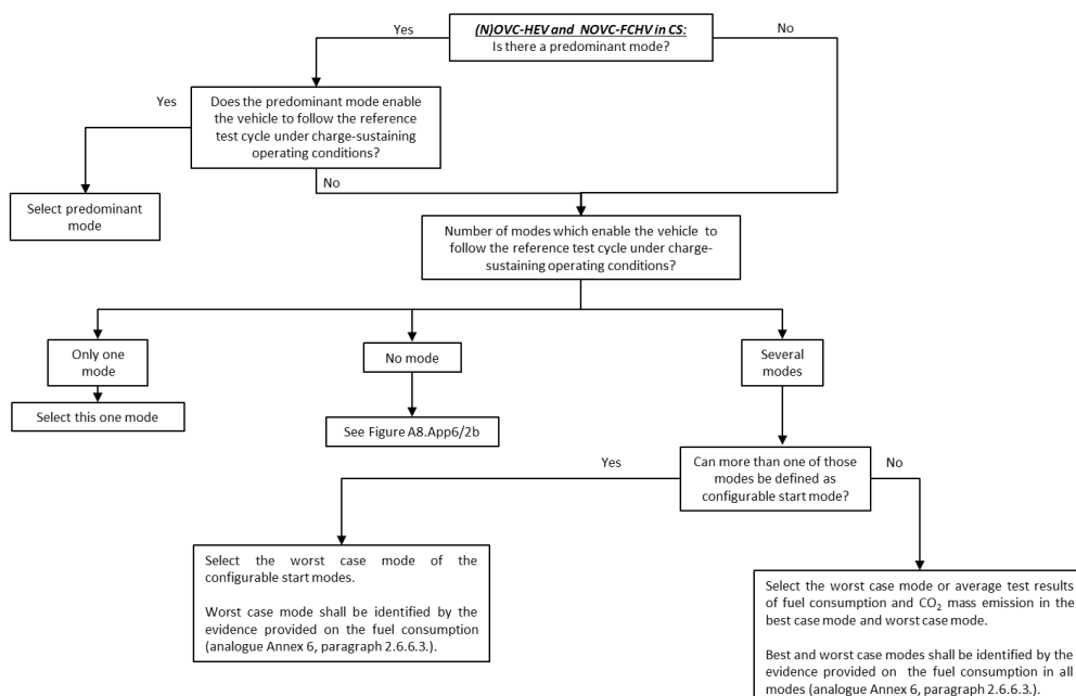
Figure A8.App6/2a (N)OVC-HEV and NOVC-FCHV: CS Type 1 Test – Mode selectable switch
