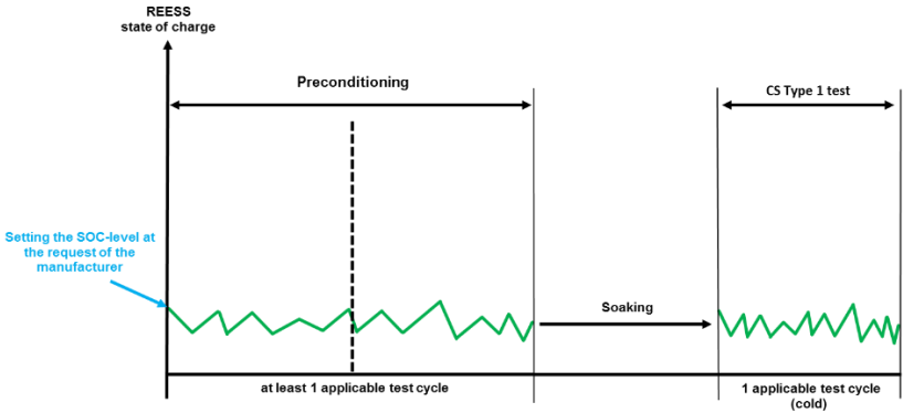
Figure A8.App1/2 OVC-HEVs, charge-sustaining Type 1 test
