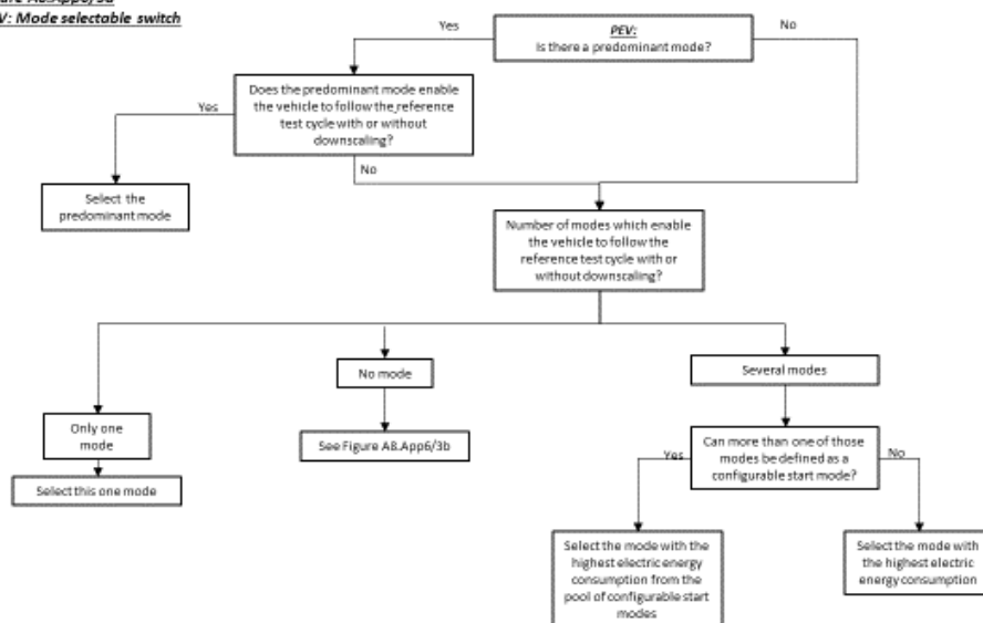
Figure A8.App6/3a PEV: Mode selectable switch
