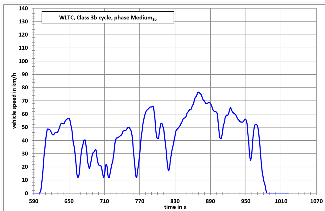
Figure A1/9 WLTC, Class 3b cycle, phase Medium 3b
