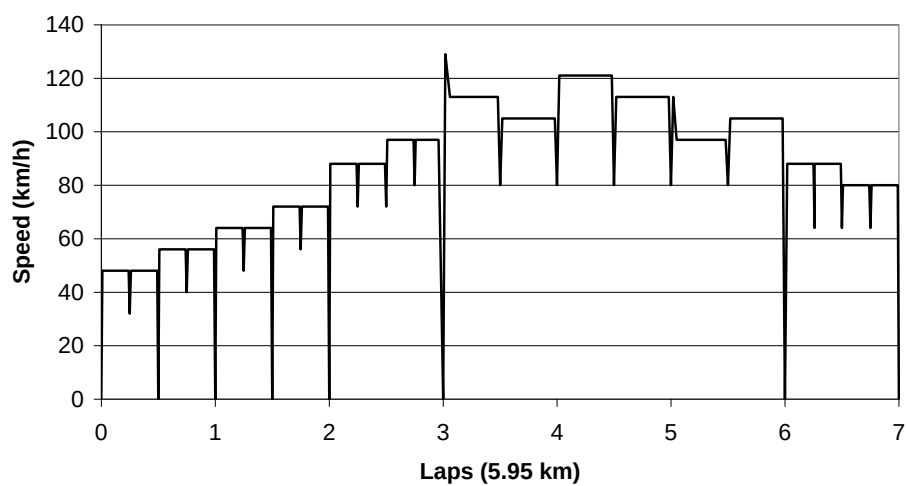
Standard Road Cycle
