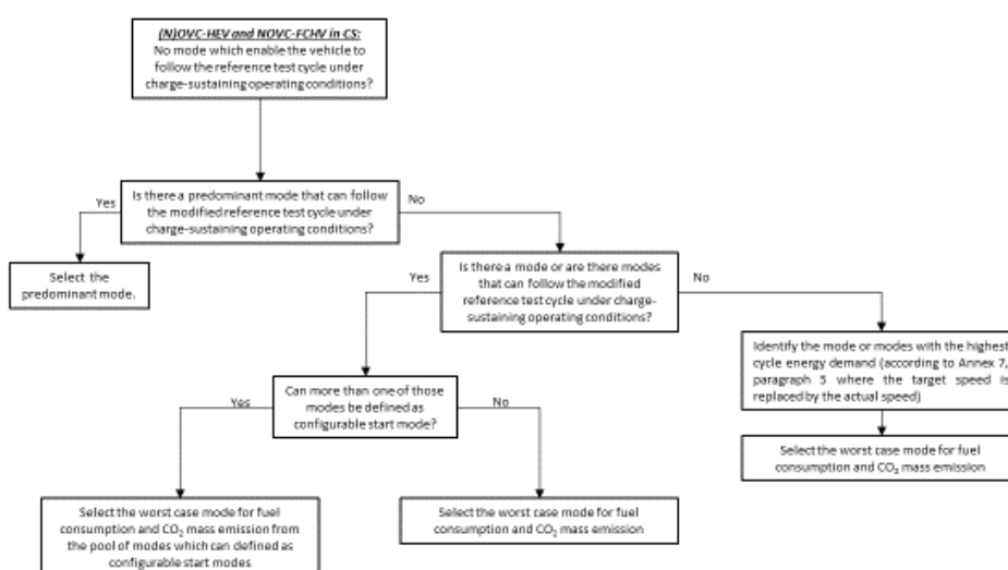
Figure A8.App6/2b (N)OVC-HEV and NOVC-FCHV: CS Type 1 Test – Mode selectable switch
