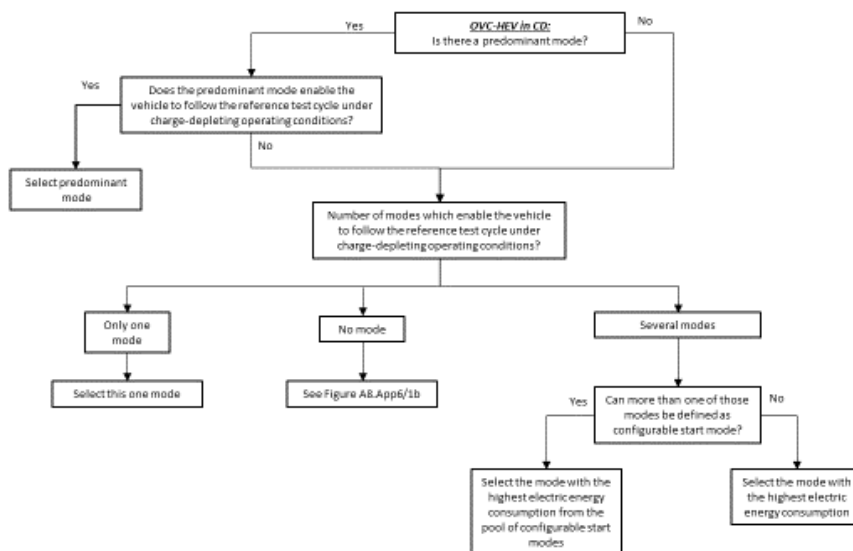
Figure A8.App6/1a OVC-HEV: CD Type 1 Test – Mode selectable switch
