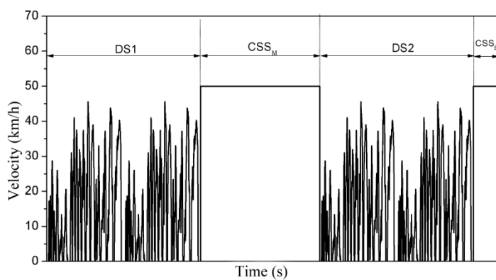
Figure A3/6 Shortened test method
