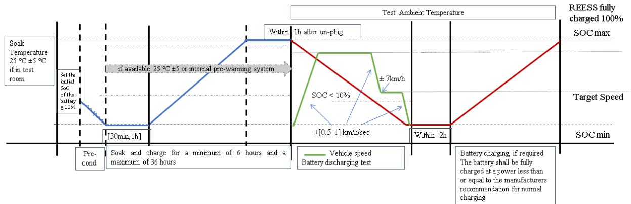
Figure A3/2 Test sequence Method 1b
