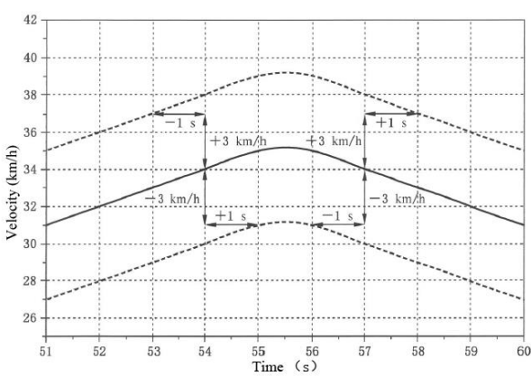
Figure A3/5 Example, reference curve and tolerance
