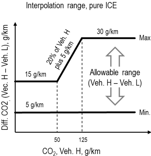
Figure A6/2 Interpolation range for pure ICE vehicles
