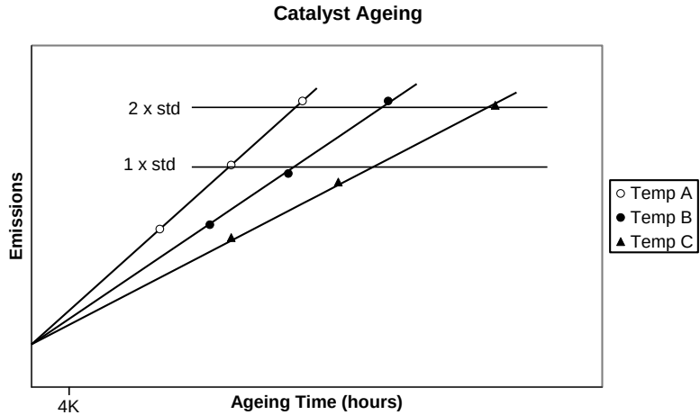
Figure C4 App1/3 Example of catalyst ageing
