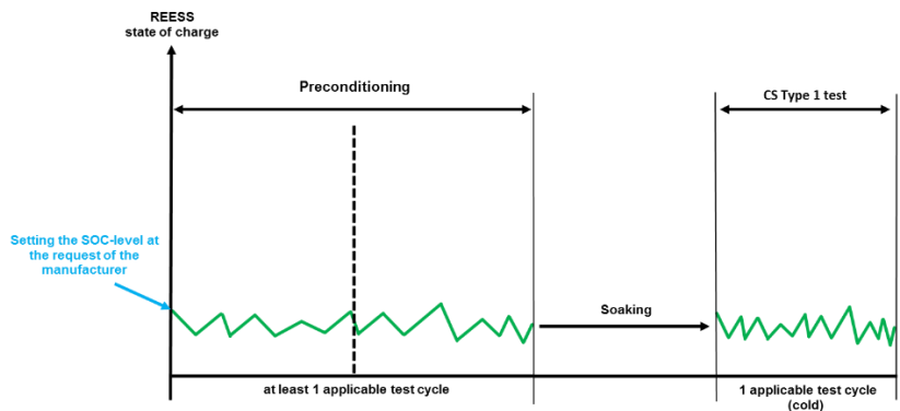
Figure A8.App1/2 OVC-HEVs and OVC-FCHVs, charge-sustaining Type 1 test
