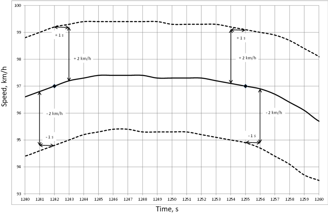
Figure A6/6 Speed trace tolerances
