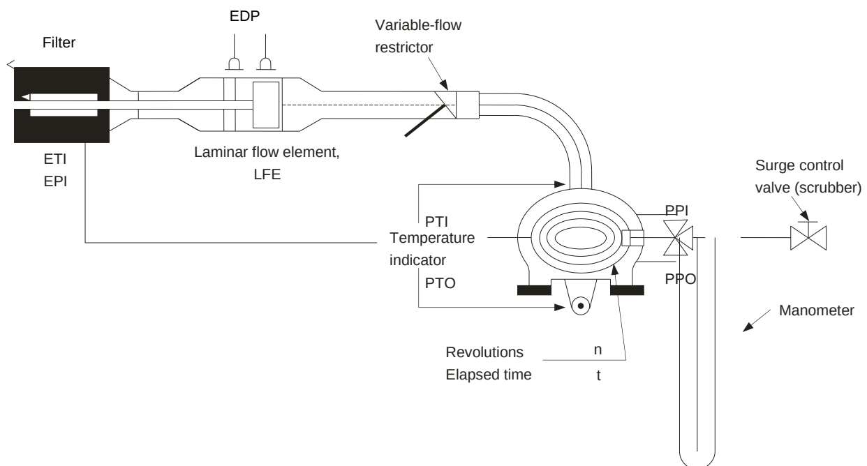
Figure A5/6 PDP calibration configuration
