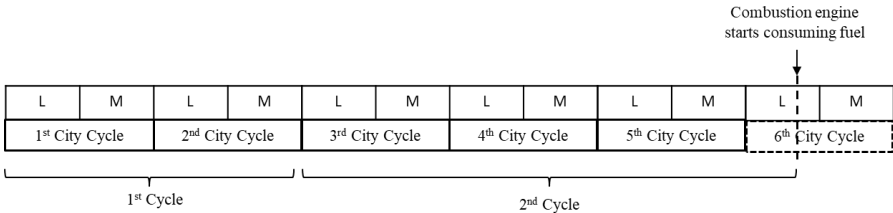
Figure A7/2 Example with an odd number of completed city test cycles before the city cycle where the combustion engine start
