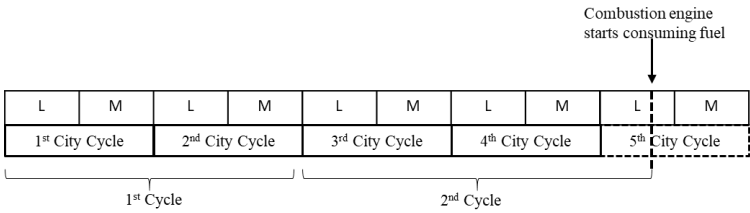
Figure A7/1 Example with an even number of completed city test cycles before the city cycle where the combustion engine start
