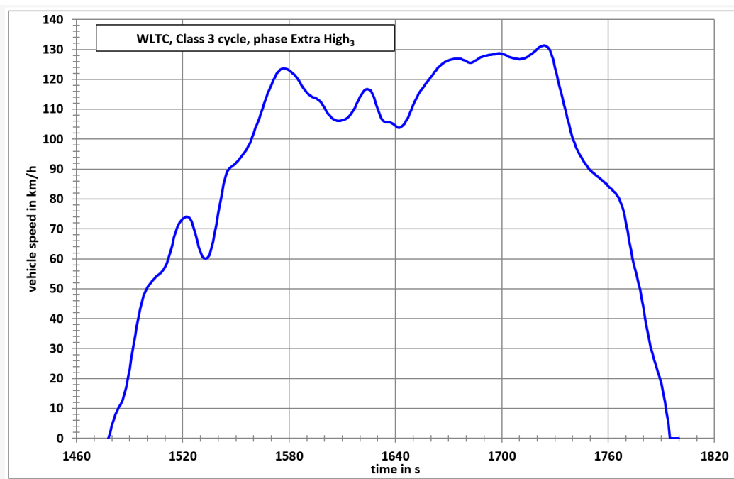
Figure A1/12 This figure is only applicable for Level 1A; WLTC, Class 3 cycle, phase Extra High 3
