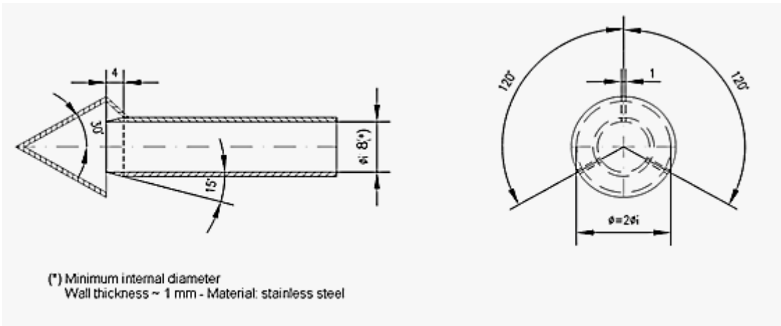
Figure A5/11 Alternative particulate sampling probe configuration
