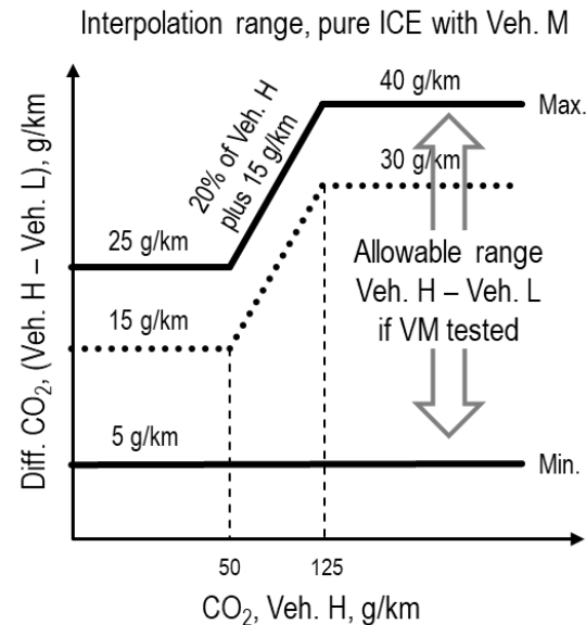
Interpolation range for pure ICE vehicles with vehicle M
