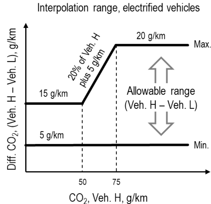
Figure A8/3 Interpolation range between vehicle H and vehicle L applied to EVs
