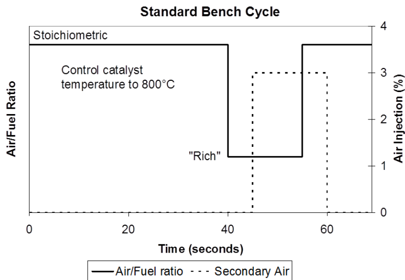
Figure C4 App1/2 Standard Bench Cycle
