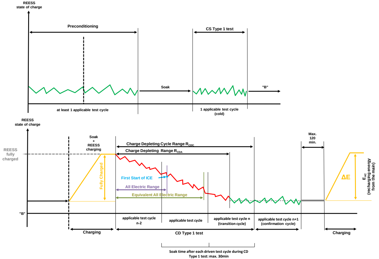
Figure A8.App1/4 OVC-HEVs and OVC-FCHVs, charge-sustaining Type 1 test with subsequent charge-depleting Type 1 test
