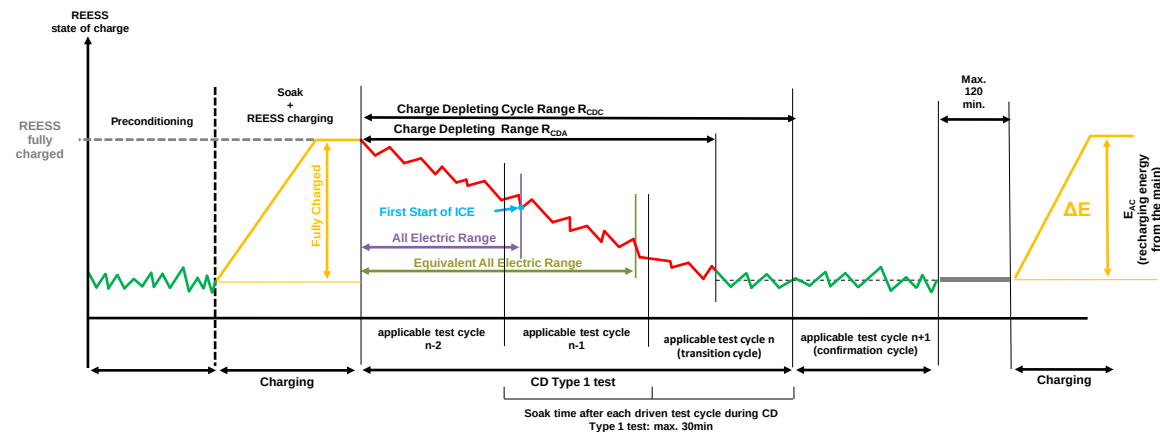
Figure A8.App1/1 OVC-HEVs and OVC-FCHVs, charge-depleting Type 1 test
