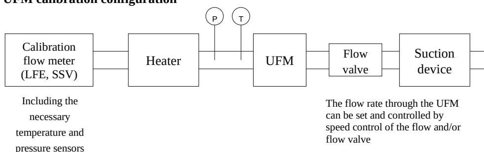
Figure A5/8 UFM calibration configuration
