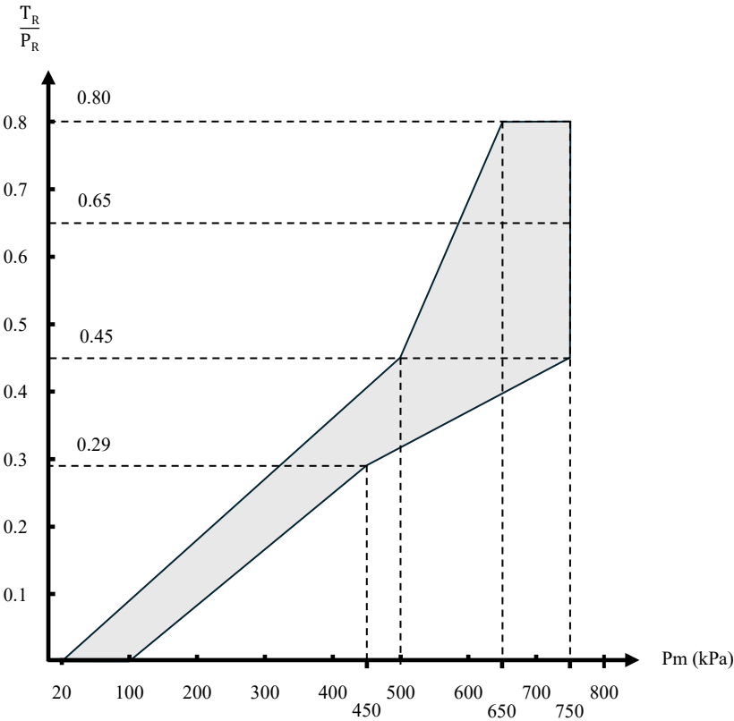
Diagram 4A Semi-trailers (see paragraph 4 of this annex)
