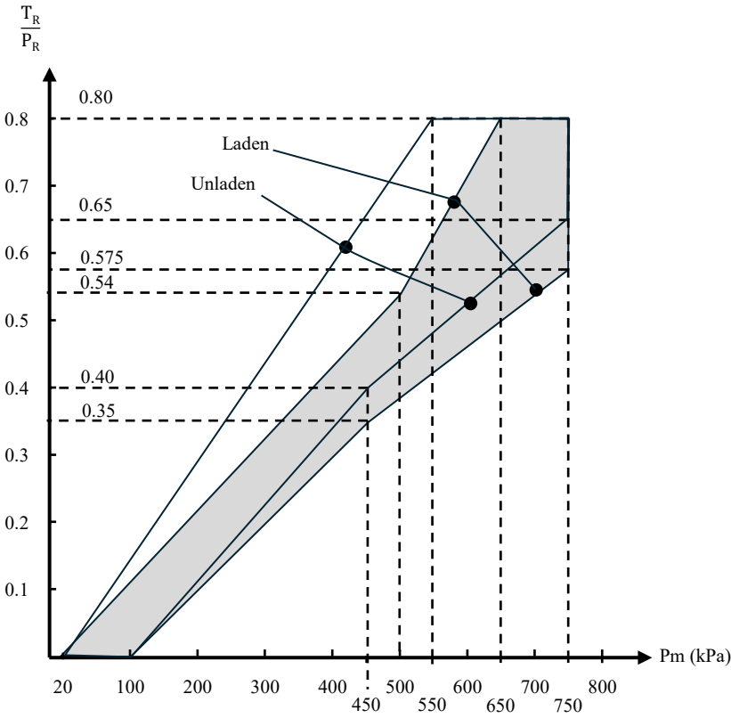
Diagram 5 Full trailers and centre-axle trailers (see paragraph 5 of this annex)
