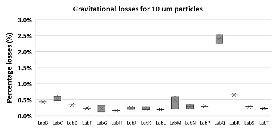
Figure 34 Percent error due to gravitational losses for 10 \mu\text{m} particles in the tunnel. The following assumptions have been considered: d_a=10 \mu\text{m} , V_{\text{settling}}=0.00304 \text{ m/s} , \rho_{\text{air}}=1.2 \text{ kg/m}^3 , \mu=1.83\text{E-}05 , L_{\text{ref}}=1 \text{ m} .
