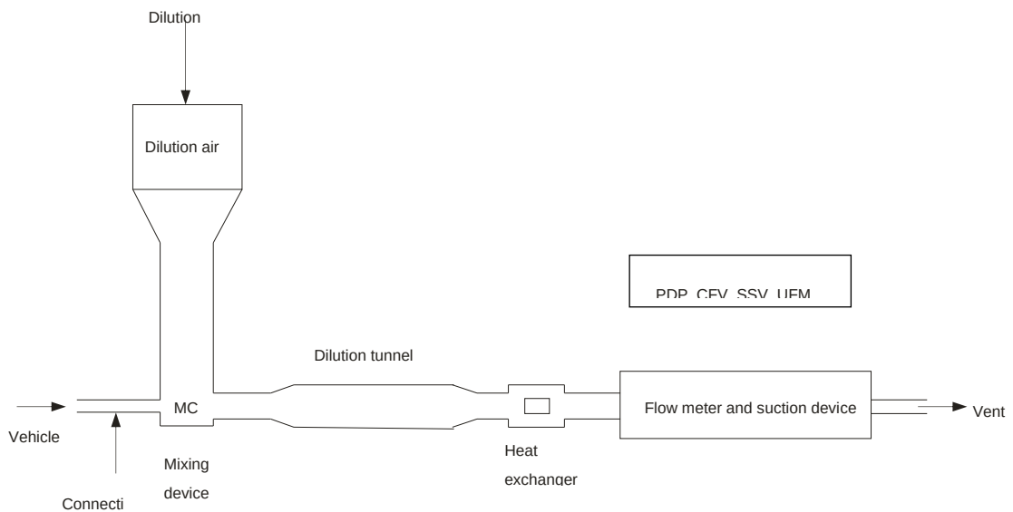
Figure A5/3 Exhaust dilution system
