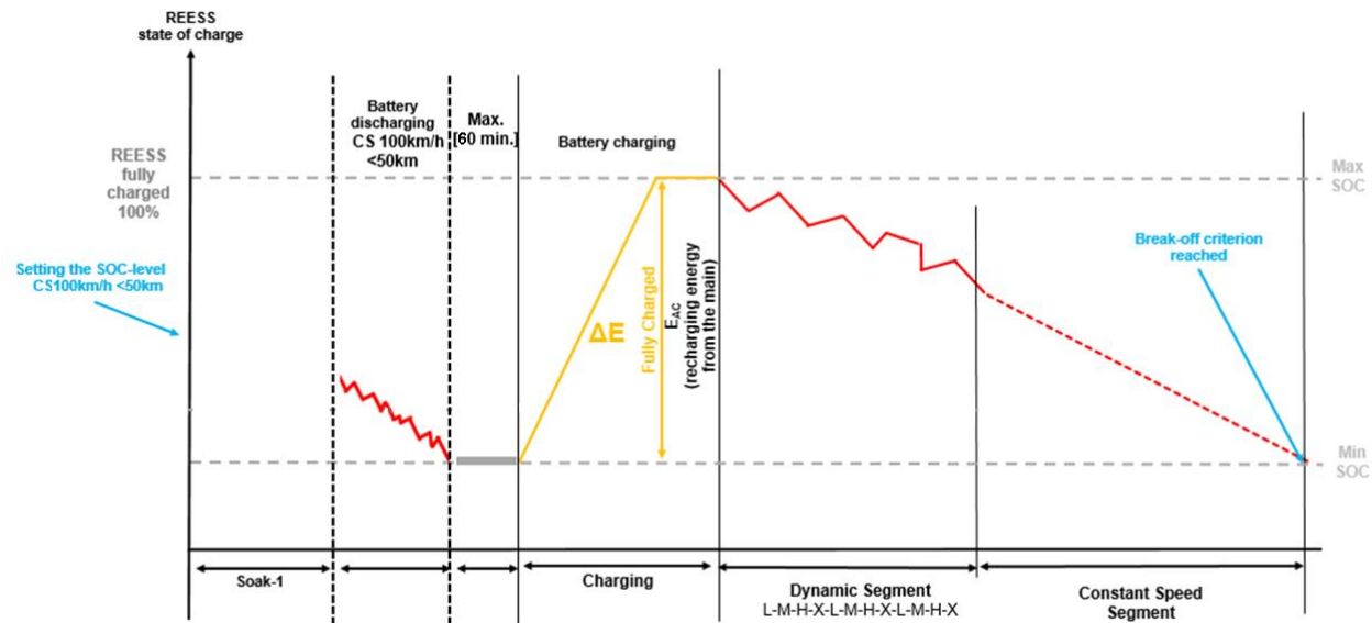
Figure B10.App1/1 PEV low temperature test sequence
