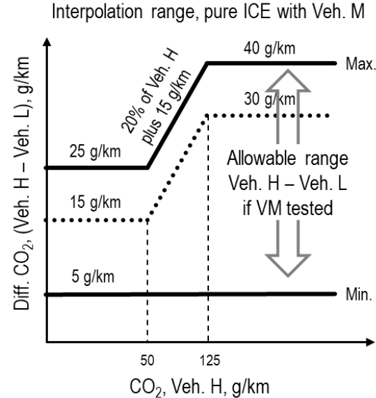
Figure A6/3 Interpolation range for pure ICE vehicles with vehicle M Interpolation range, pure ICE with Veh. M
