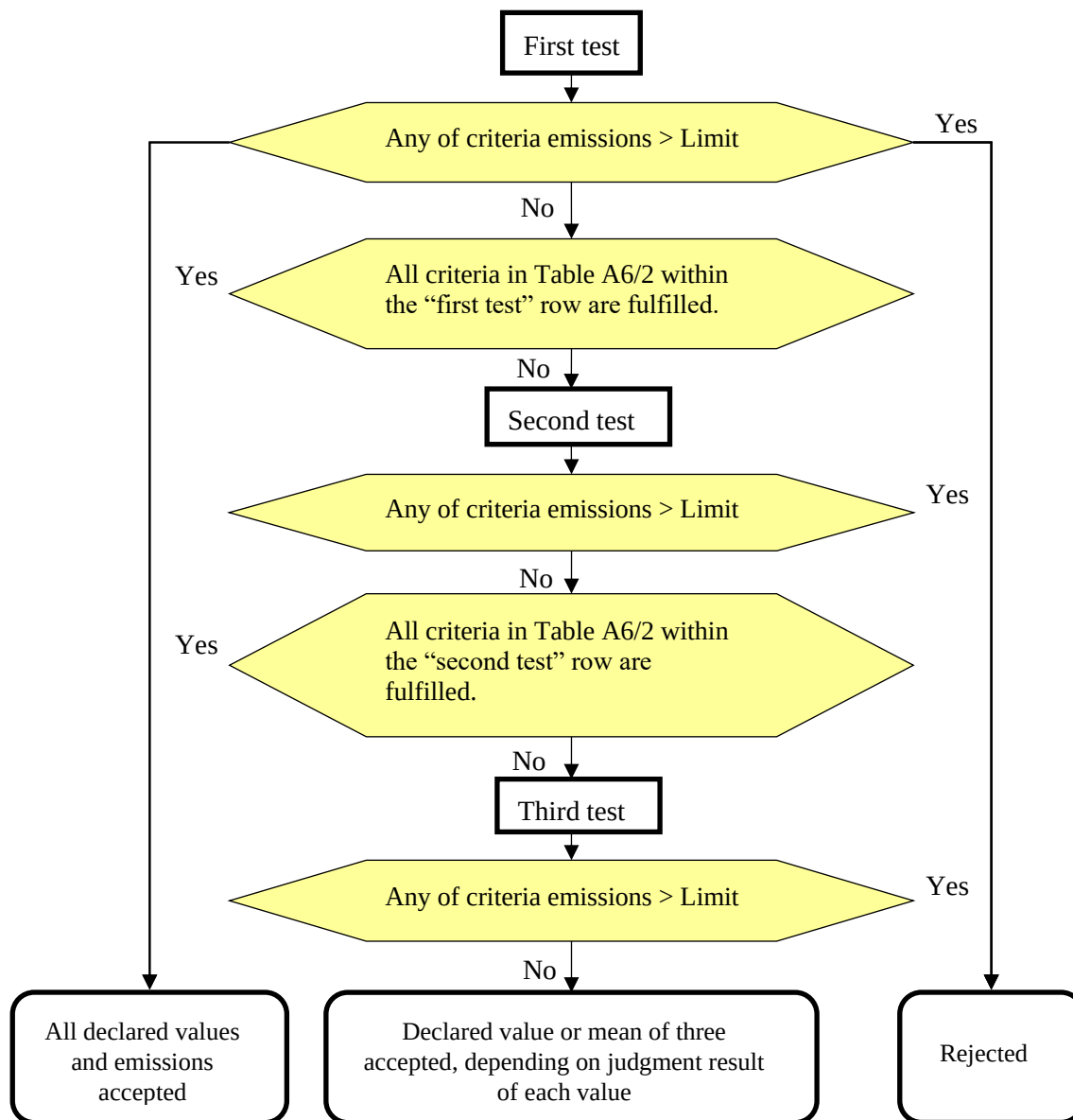
Figure A6/1 Flowchart for the number of Type 1 tests
