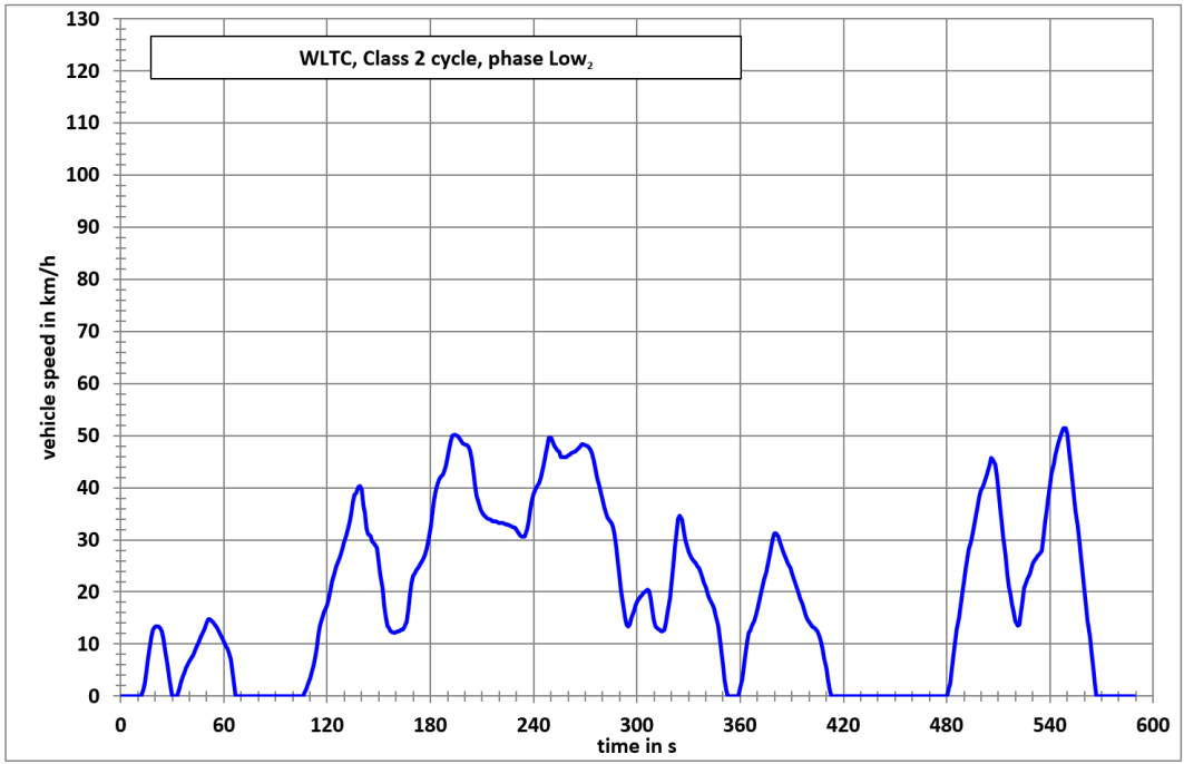
Figure A1/3 WLTC, Class 2 cycle, phase Low 2
