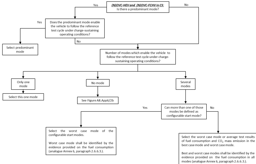
Figure A8.App6/2a (N)OVC-HEV and (N)OVC-FCHV (as applicable): CS Type 1 Test – Mode selectable switch
