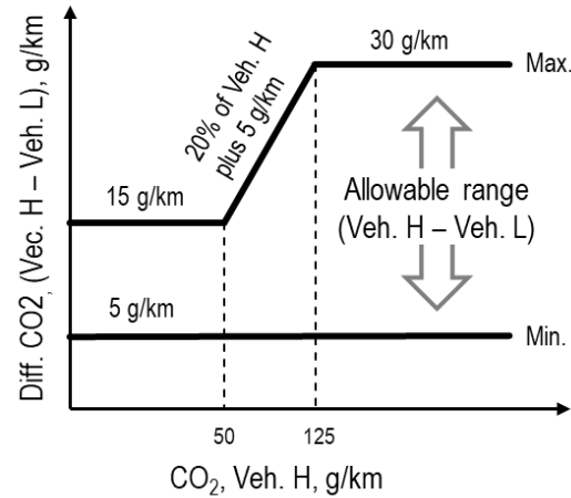
Figure A6/2 Interpolation range for pure ICE vehicles Interpolation range, pure ICE
