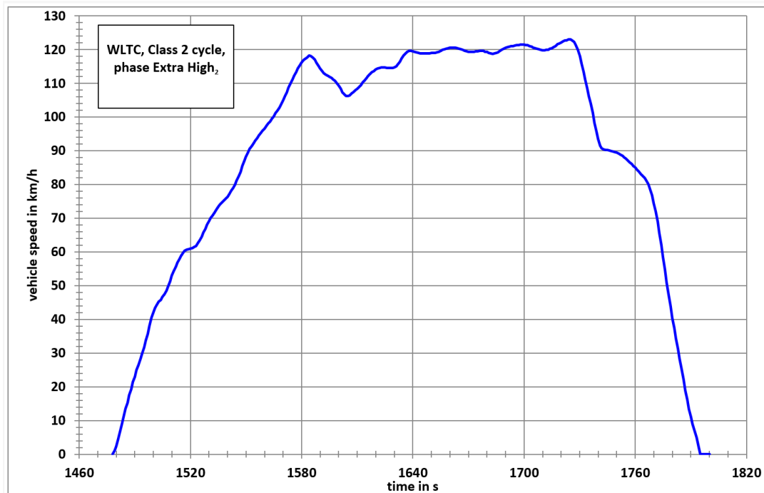
WLTC, Class 2 cycle, phase Extra High 2
