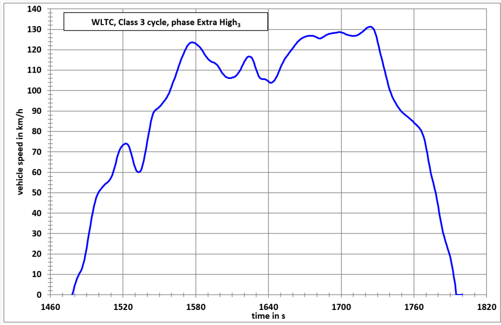
Figure A1/12 This figure is applicable to Level 1A and 4-phase WLTP test in Level 2 only; WLTC, Class 3 cycle, phase Extra High 3
