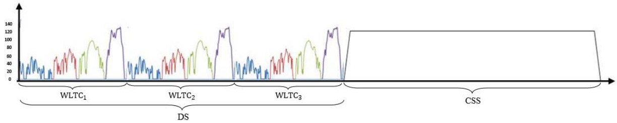
Figure B10/1 PEV Low Temperature test procedure speed trace
