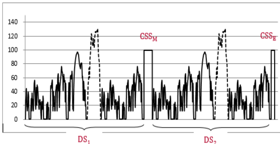
Figure A8/2 Shortened Type 1 test procedure speed trace
