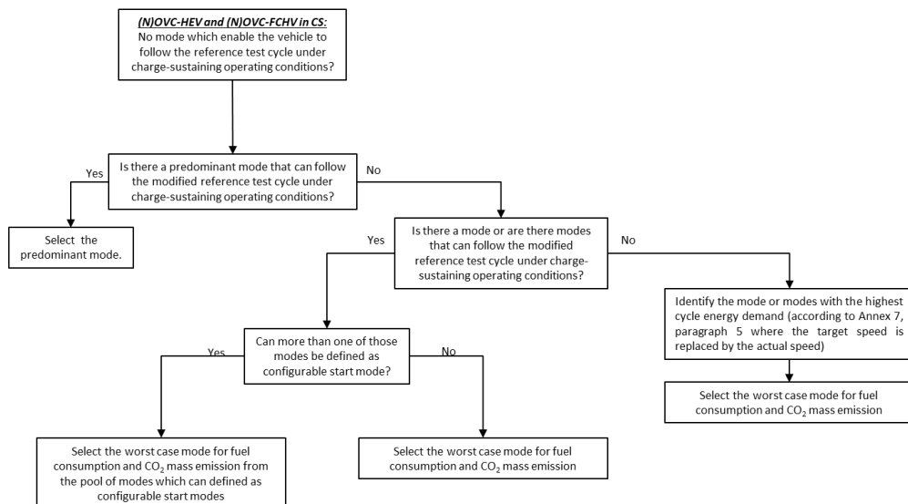
Figure A8.App6/2b (N)OVC-HEV and (N)OVC-FCHV (as applicable): CS Type 1 Test – Mode selectable switch
