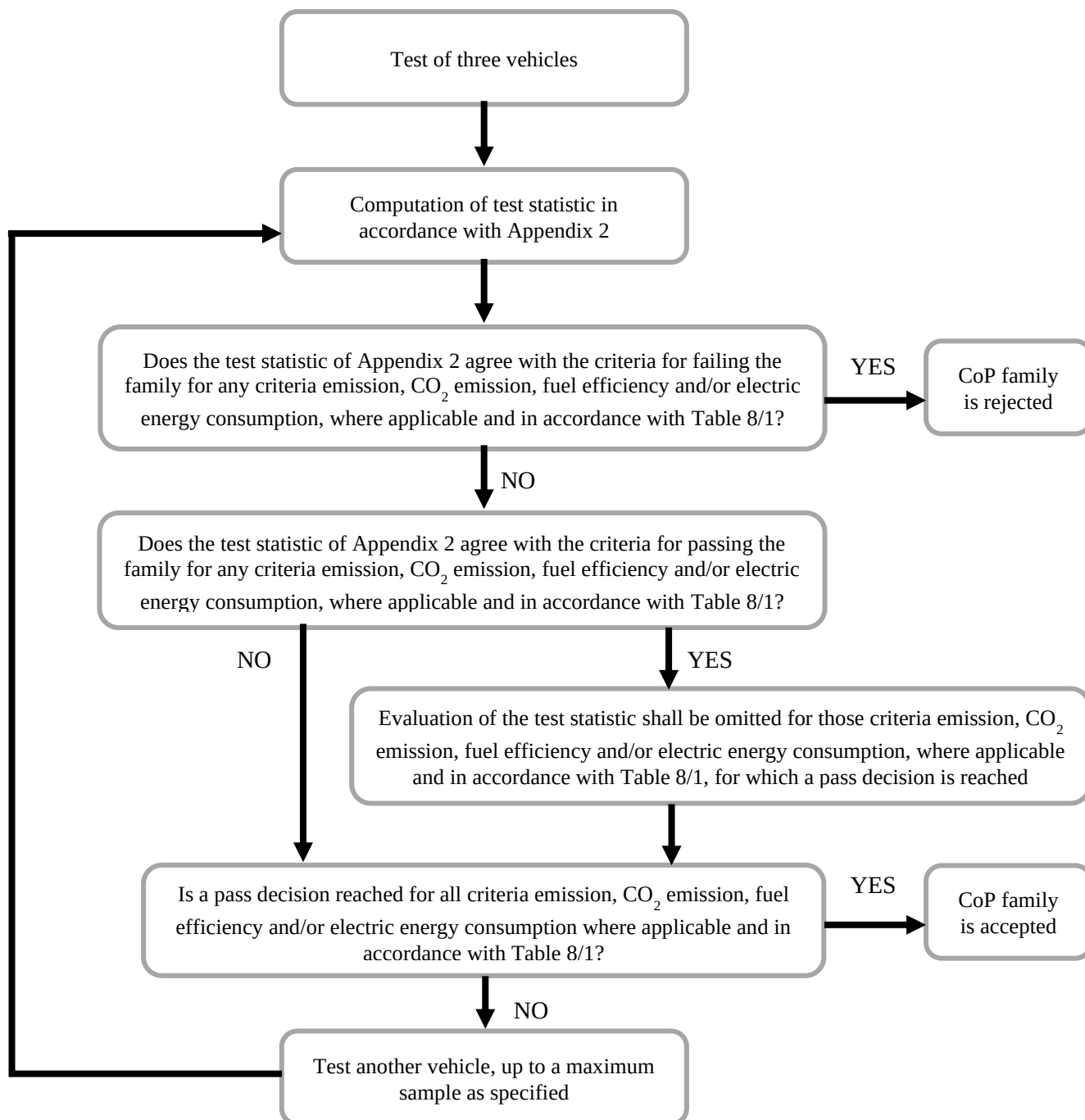
Figure 8/1 Flowchart of the CoP test procedure for the Type 1 test
