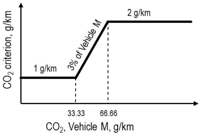
Figure A6/5 Linearity criterion for vehicle M Tolerance, Vehicle M measured vs. calculated
