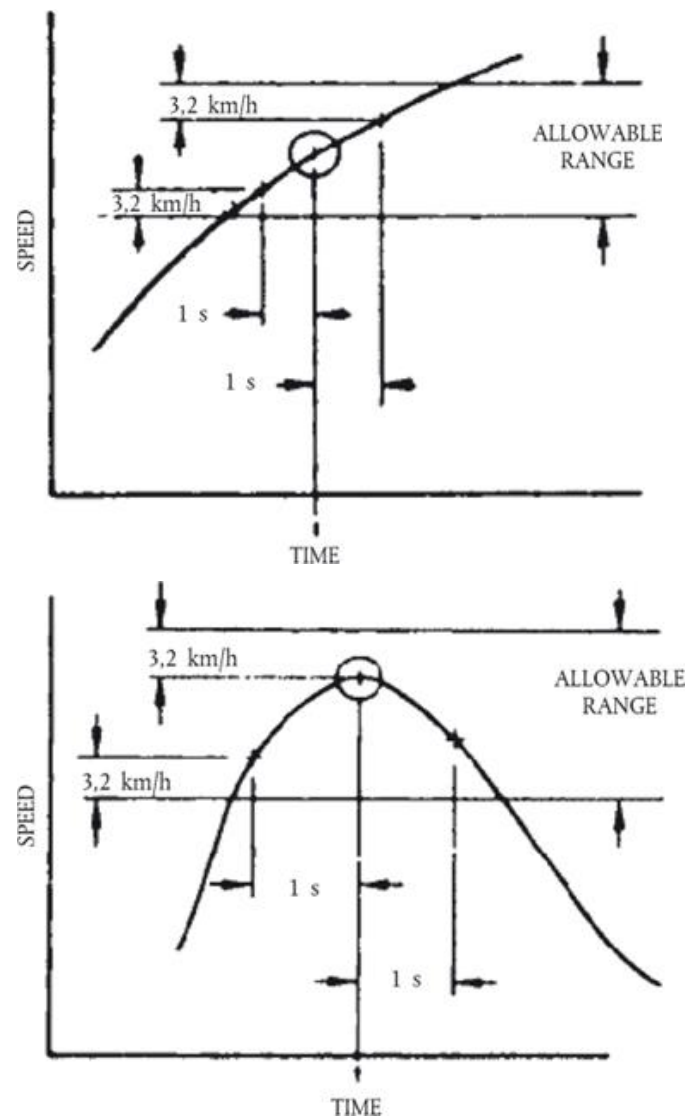
Figure A4/2: Drivers trace, allowable range
