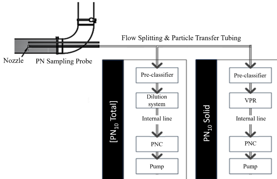
Indicative setup of the PN sampling and measurement unit
