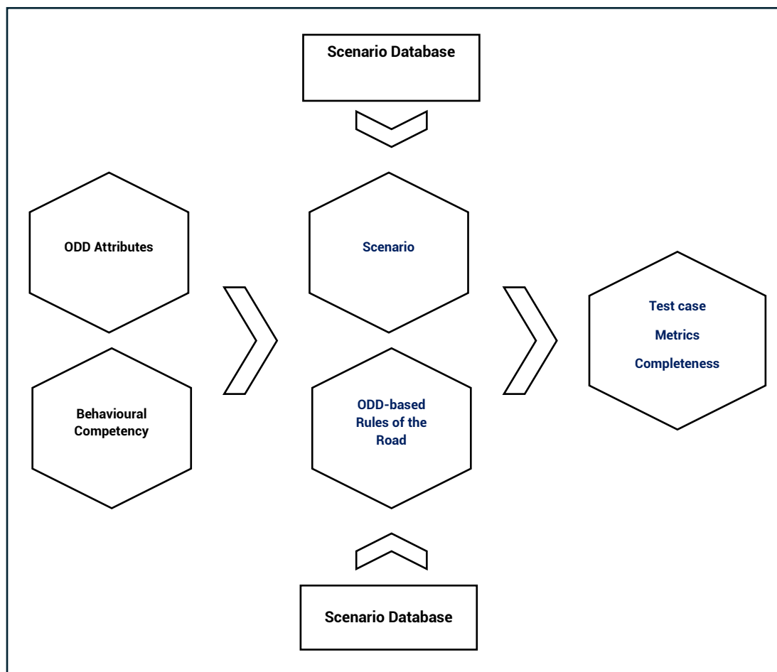
Figure 3. Rules of the road as pass/fail criteria
