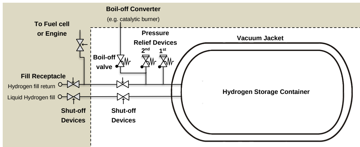
Figure 1 Typical liquefied hydrogen storage system
