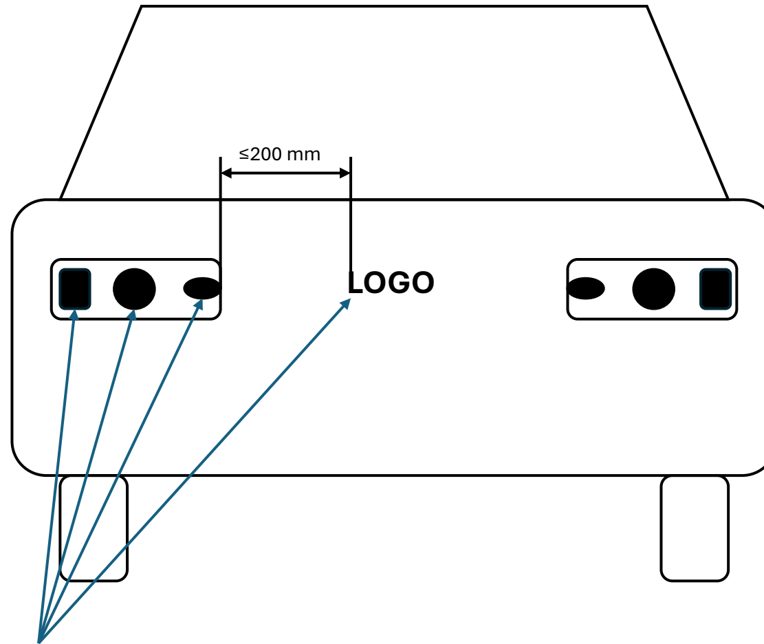
Lighting units of an AFS
