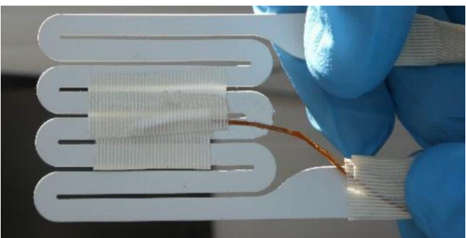
Figure 2 Example of Placement of the Temperature Sensor on the Heater Element
